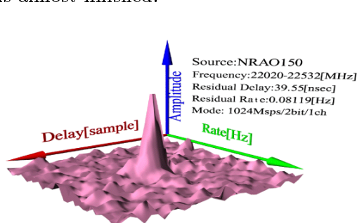
Figure 2. 2 Gbps fringes observed on Kashima - Metsähovi baselline using K5/PC-VSI system.
