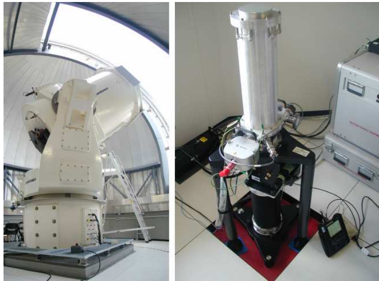
Figure 2. MLRO Telescope and Absolute Gravimeter.
